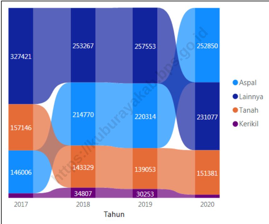
Gambar 8 Panjang Jalan Kabupaten Menurut Jenis Permukaan di Kabupaten Kubu Raya, 2017-2020 Length of Regency Roads by Type of Surface in Kubu Raya Regency, 2017-2020
